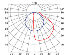
— C0-C180 — C90-C270 Transparent cover
