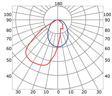
— C0-C180 — C90-C270 60° lens cover (light reduction: -17%)
