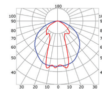
Transparent cover (light reduction -35%)
