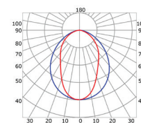
Semiopal cover (light reduction -42%)
